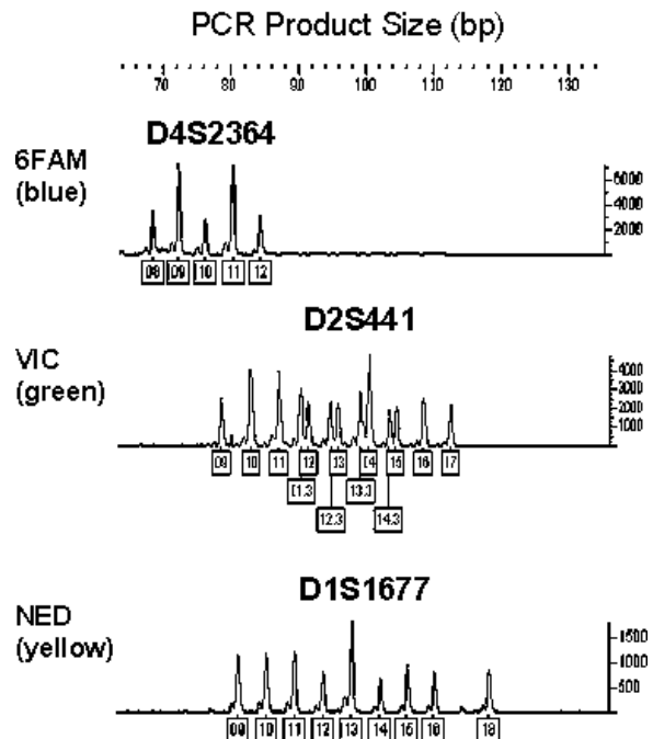
FIG. 3—MiniSTR allelic ladders for miniplex01 (top panel) and miniplex02 (bottom panel). Samples were amplified individually and electrophoretically separated on an ABI 310.
