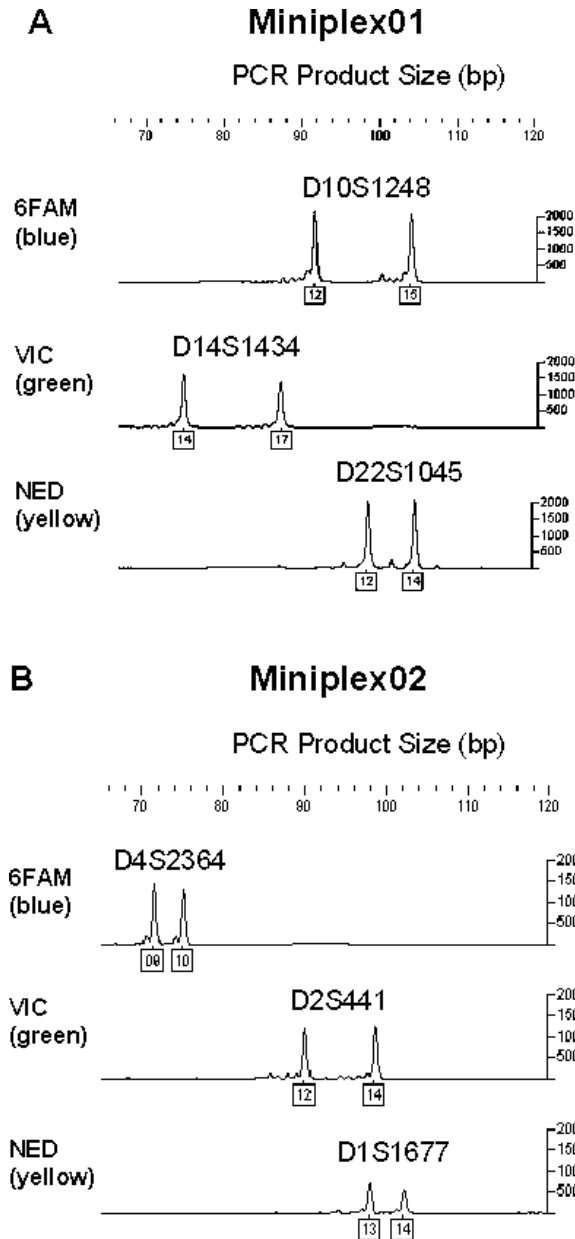
FIG. 2—Representative sample from an individual analyzed with both (A) miniplex01 and (B) miniplex02 using standard conditions for amplification (28 cycles, 1U AmpliTaq Gold polymerase, 10 \mu L PCR).
