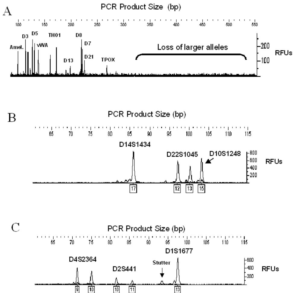
FIG. 5—Comparison of STR allele peak heights obtained from (A) PowerPlex ® 16, (B) miniplex01 and (C) miniplex02 loci with equivalent amounts of the same degraded bone sample (approximately 6 pg/ \mu L quantified using real time PCR—Denise Chung, personal communication). All samples were amplified for 32 cycles of PCR with 2U of AmpliTaq Gold polymerase in a 25 \mu L volume. Peak heights are in relative fluorescence units (RFUs).
