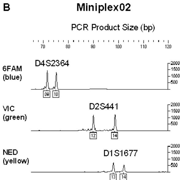
FIG. 2—Representative sample from an individual analyzed with both (A) miniplex01 and (B) miniplex02 using standard conditions for amplification (28 cycles, 1U AmpliTaq Gold polymerase, 10 \mu L PCR).
