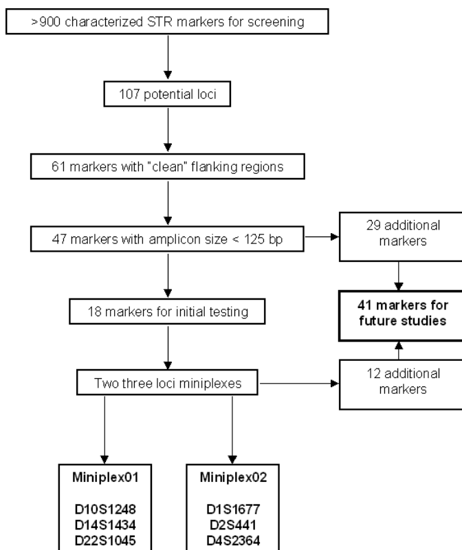
FIG. 1—Schematic of the screening process to identify miniSTR loci. Published STR markers (23, 28–30) were used to screen for “ideal” markers to make small amplicons. In general, potential loci were selected for allele ranges less than 24 bp and heterozygosity values greater than 0.70.
