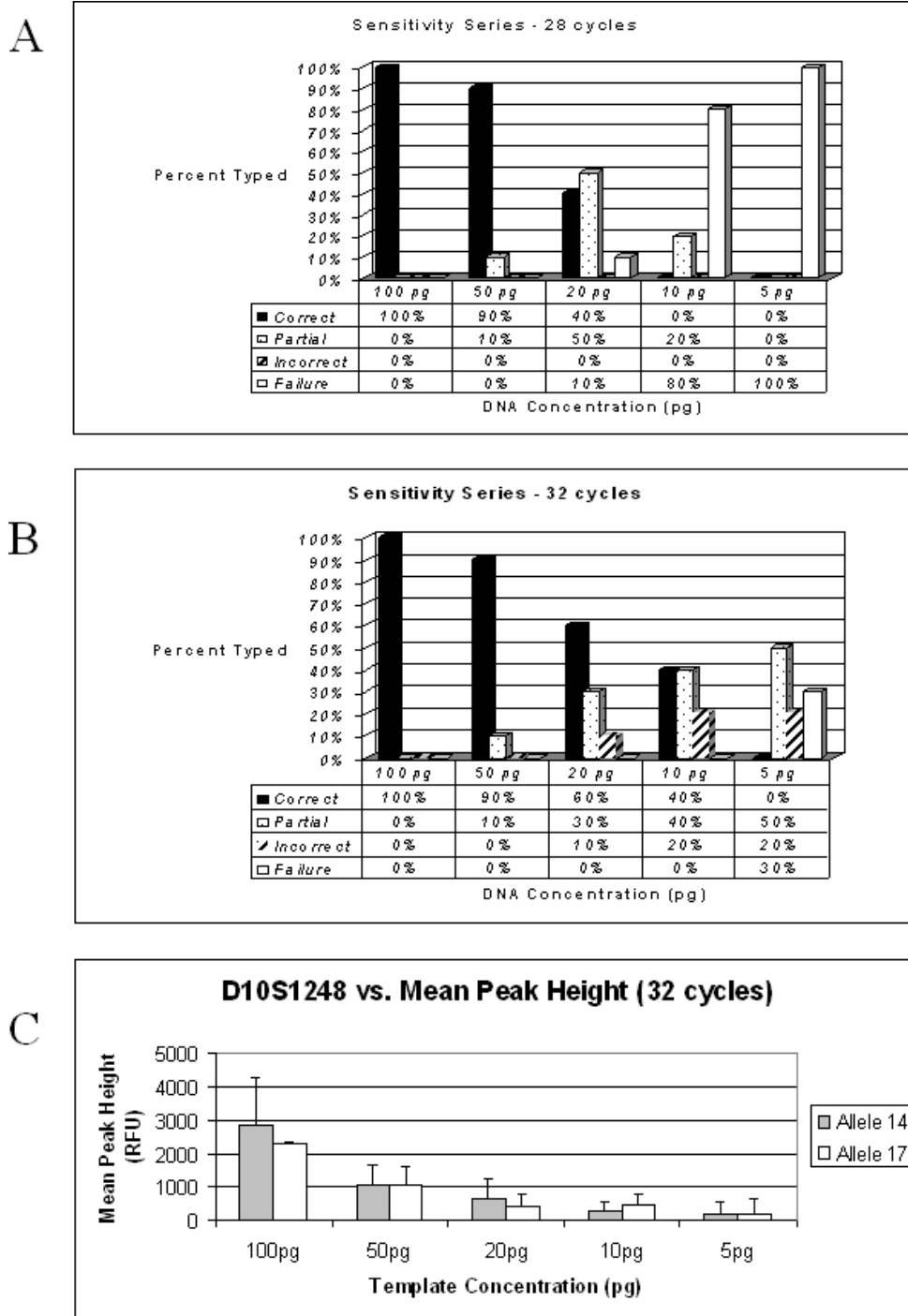
FIG. 4—Sensitivity results for DNA dilutions using the D10S1248 marker. Results are from 10 replicate PCR amplifications and were analyzed on the ABI 3100. An interpretational threshold of 50 relative fluorescent units (RFUs) was used for genotyping each dilution. Each replicate was typed as being either correct (matching the genotype at 1 ng amplification), partial (one allele in a heterozygote drops below 50 RFUs), incorrect (allele drop-in that creates a wrong genotype), or failure (no peaks were observed above 50 RFUs). (A) Results with 28 cycles of PCR amplification and 1U of DNA polymerase. (B) Results with 32 cycles of PCR amplification and 2U of DNA polymerase. These results show an increase in the successful typing at low template levels. However, the number of partial profiles and profiles having the incorrect typing can be increased with extra samples and extra polymerase. (C) Mean Peak Height values from samples amplified at 32 cycles with 2U AmpliTaq Gold polymerase for the D10S1248 marker.
